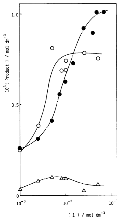
Fig. 2. Dependence of yields of 3 and 4 under N_2 and 2 under O_2 on the concentration of 1 .
