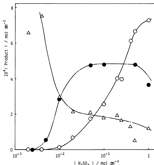
Fig. 1. Dependence of photo-methoxylation and -hydroxymethylation at the 2-position under N_2 and photo-methoxylation at the 3-position under O_2 on the concentration of sulfuric acid.
